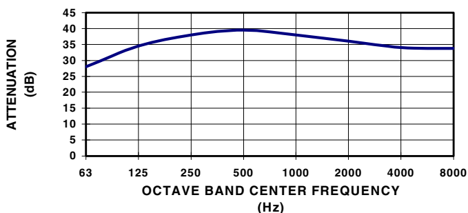
REPRESENTATIVE ATTENUATION CURVE FOR "JH" SERIES SILENCER
