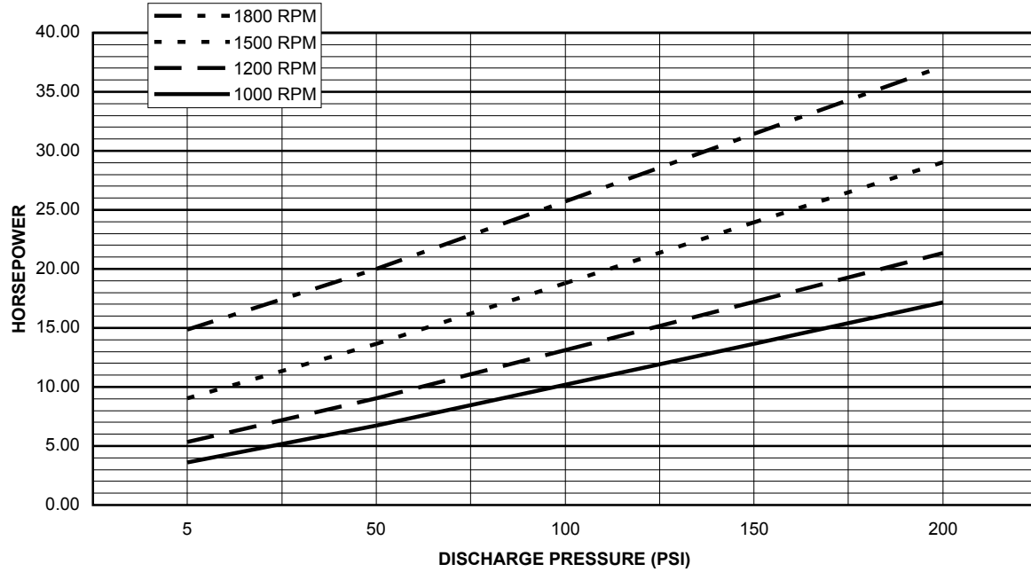
PUMP WATER HP VERSUS DISCHARGE PRESSURE EDWARDS MODEL 150-348 STANDARD DUTY
