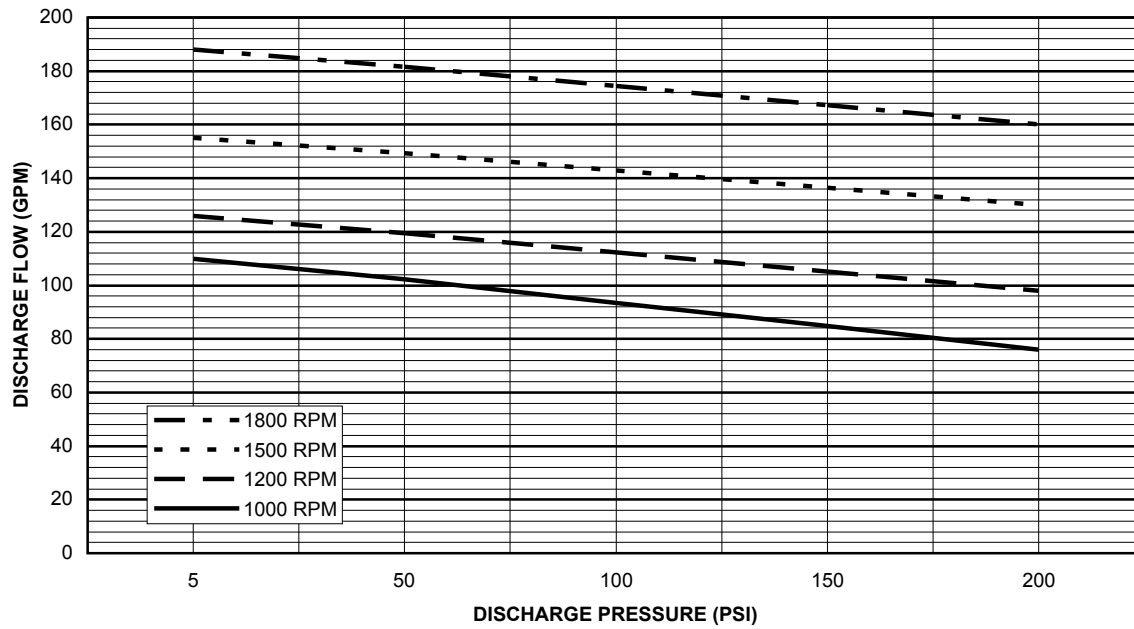
PUMP WATER FLOW VERSUS DISCHARGE PRESSURE EDWARDS MODEL 150-348 STANDARD DUTY
